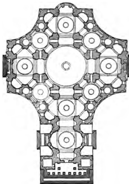
PLAN OF ST. PAUL'S AS FIRST DESIGNED BY WREN.
